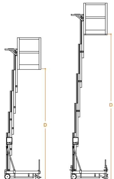
WITHOUT STABILIZERS
